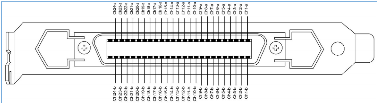
Fig.1, 5001L01, 5001L02, 5001L03_Parallel, 2-wire pin-out
