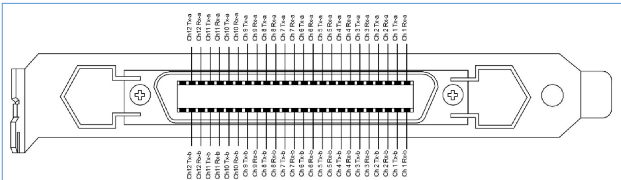
Fig.1, 5001L01, 5001L02, 5001L03_Parallel, 4-wire pin-out
